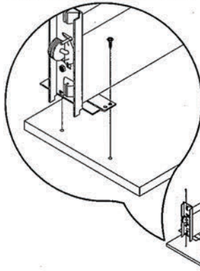
Screw s1 Ø4x14mm (x4)
